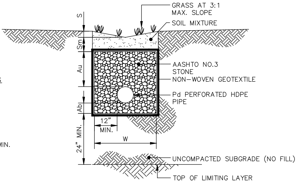
SECTION VIEW
