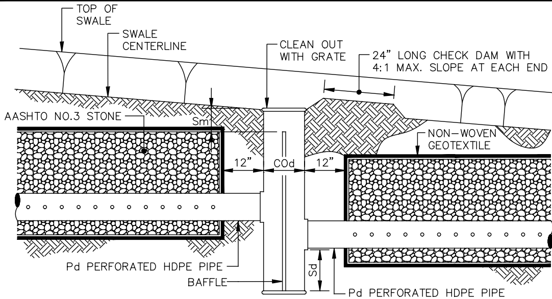
PROFILE VIEW
