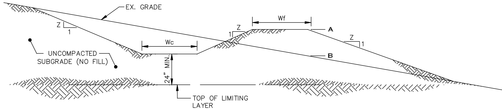
SECTION VIEW
