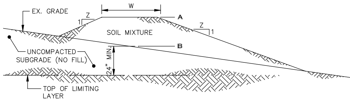
SECTION VIEW
